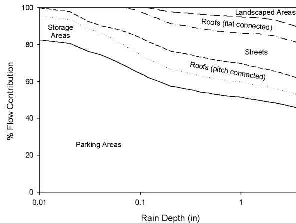
Figure 16.1 Flow sources for example commercial/mall area (Bochis 2007).
