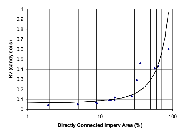
Figure 16.5 Relationships between the directly connected impervious area (%) and the calculated volumetric runoff coefficients (Rv) for each land use category for sandy soil (Bochis and Pitt 2005)
