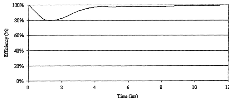
Figure 19.6 Vortechs™ system total suspended solids (TSS) removal on Jan. 20, 1995.
