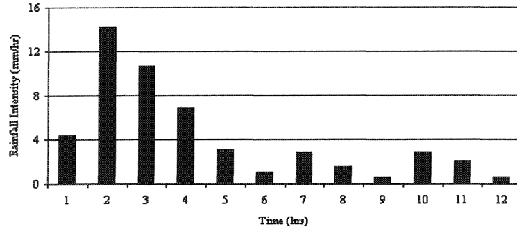
Figure 19.1 Rainfall hyetograph for a January 20, 1995 event in southeast Cumberland County, Maine.
