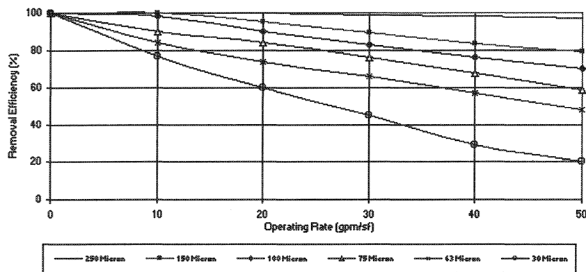
Figure 19.5 Uniform particle removal efficiency for Vortechs™ system.
