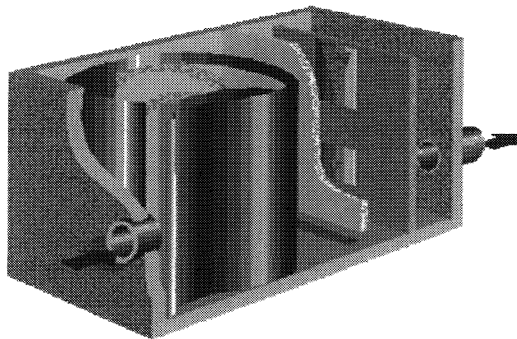
Figure 19.4 Vortechs™ stormwater treatment system - cutaway view.
