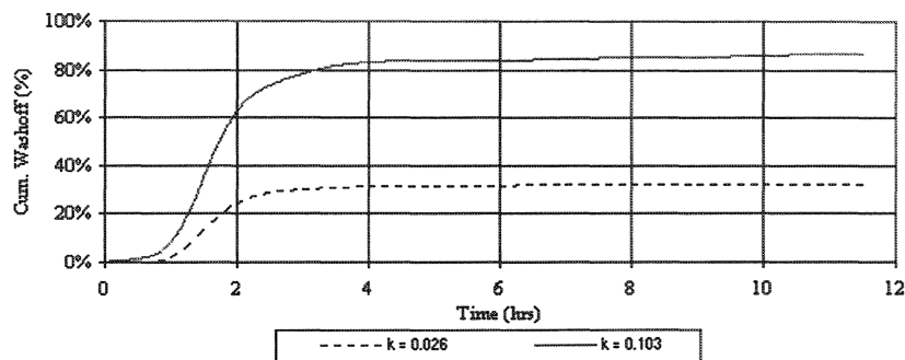
Figure 19.3 Sediment washoff for a 6-month storm in southeast Cumberland County, Maine.
