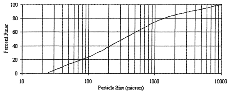
Figure 19.2 Particle size distribution of street refuse before sweeping (Pitt, 1979).
